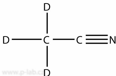
ACETONITRIL D3
