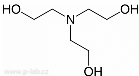
TRIETHANOLAMIN
