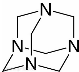
HEXAMETHYLENTETRAMIN
